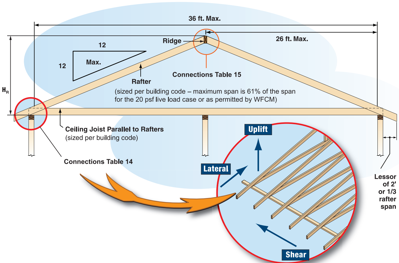
Figure 20. Roof Systems
